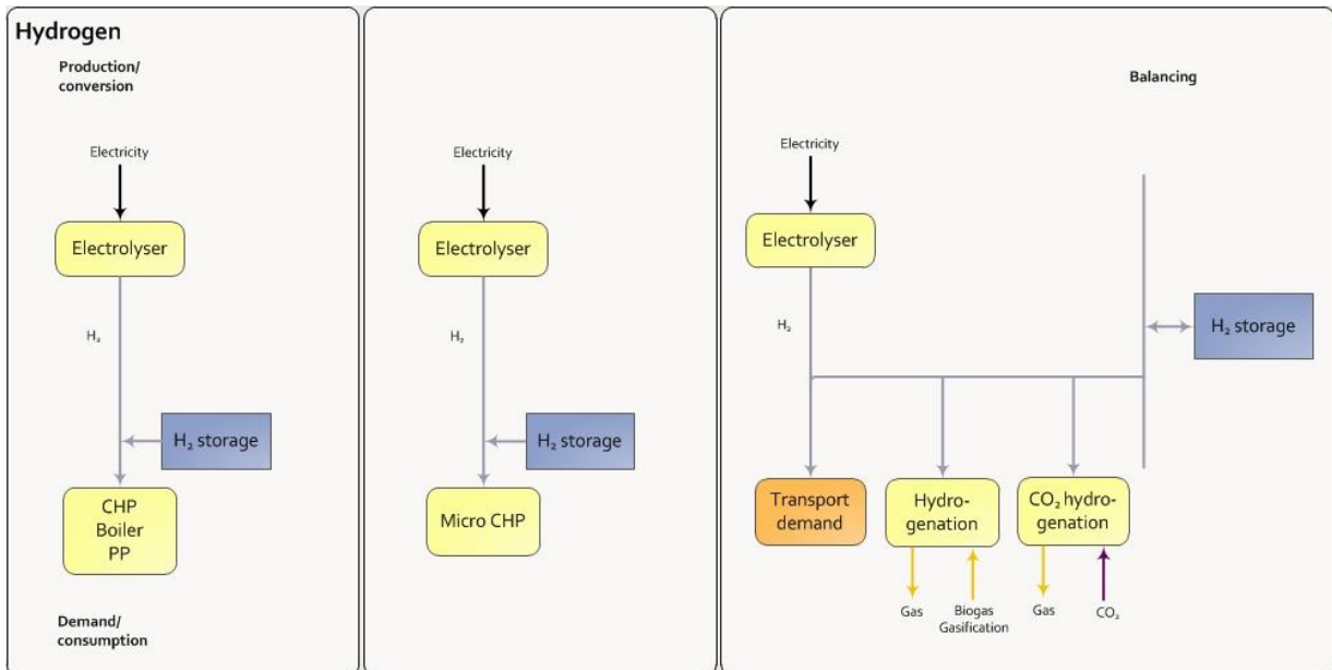
Illustration of components involved when the EnergyPLAN model calculates hourly balancing of the HYDROGEN system including interactions with other parts of the whole system. In the model, Hydrogen is calculated as three separate systems: One for CHP and Power plants; one for micro CHPs, and a joint system for the production of hydrogen for transportation and hydrogenation.
